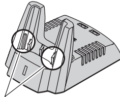
Align the slots of the battery pack with the guides in the nest of the CD-31 Desktop Rapid Charger.
