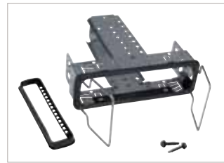
RLN4781 Direct in dashboard (DIN) mounting kit allows you to discreetly fit your radio in the dashboard.
