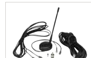
GMAE4290 Combined TETRA and GPS antenna for digital car kit operating in the 380-430MHz frequency range - includes duplexer and DC adapter. Compatible with car kit FTN6307.
