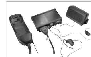
GMLN4687 Hands-free digital car kit including cradle, junction box, external speaker, remote microphone, velcro PTT and cable, 12 to 24V compatibility. Requires external antenna GMAE4290.
