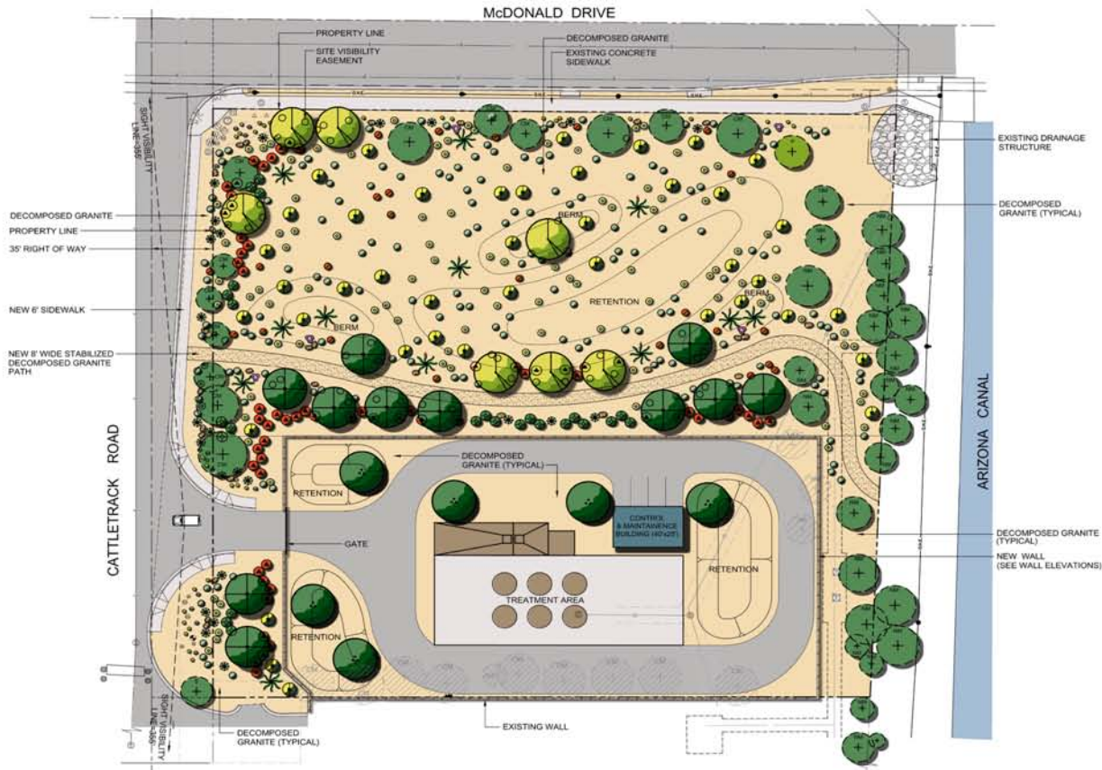
LANDSCAPE CONCEPT PLAN 5985 NORTH CATTLETRACK ROAD
