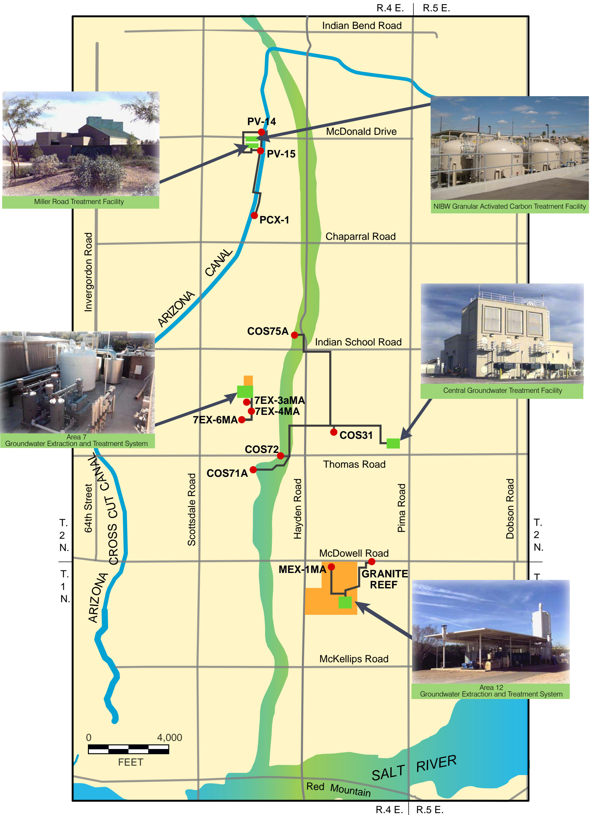
FIGURE 17. LOCATIONS FOR ACTIVE EXTRACTION WELLS, PIPELINES, AND TREATMENT FACILITIES, NIBW SUPERFUND SITE
